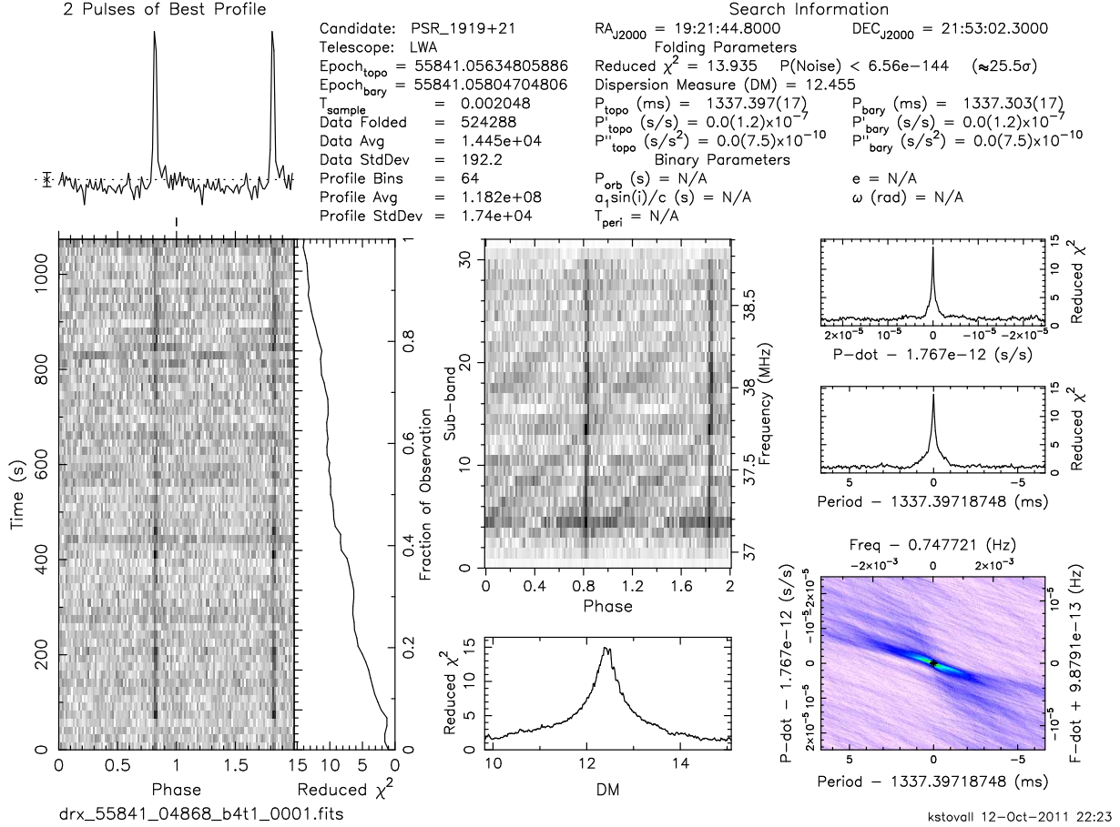
Fig. 8.— First LWA1 detection of the pulsar B1919+21 in a 1 MHz beam taken during commissioning observations. The pulsar observations were processed using PRESTO (Ransom 2001).
