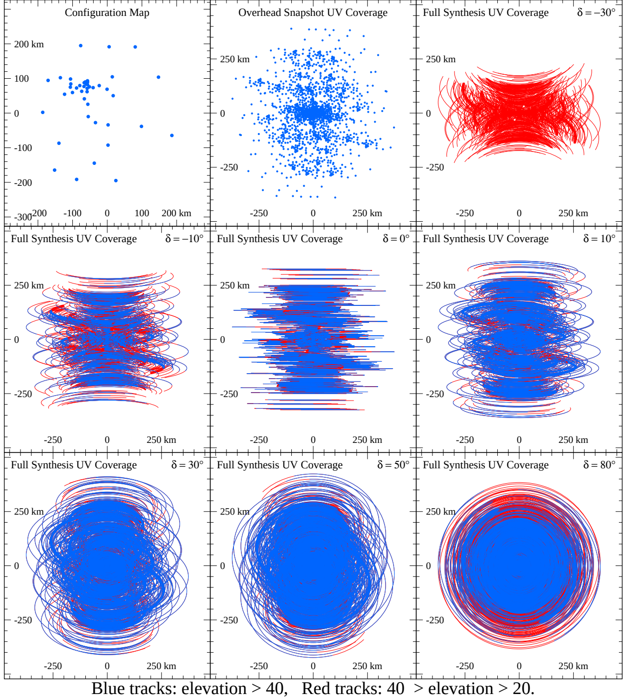
Fig. 4.— Complete LWA uv -coverage at various declinations.
