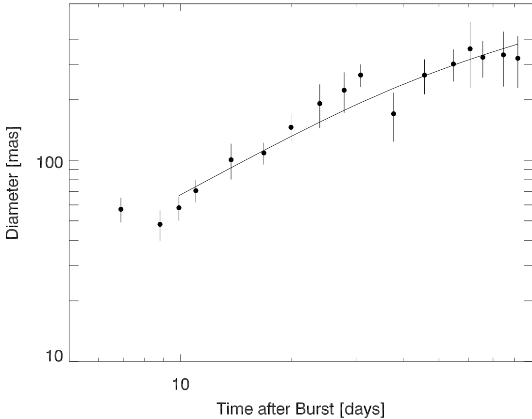
Fig. 2.— Expansion of the radio afterglow from SGR 1806-20 as a function of time. The size shown is the geometric mean of the major and minor axes of the best fitting elliptical Gaussian for each observation. The solid line is a fit of a supersonically expanding shell model as described by Eq. 4 of Gelfand et al. (2005). This model does not take into account the collimation and proper motion of the source, but provided that these are not extreme, it illustrates the deceleration due to mass loading by the external medium.
