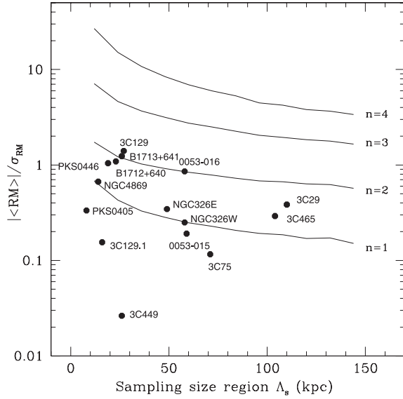
Fig. 11. The ratio |\langle \text{RM} \rangle|/\sigma_{\text{RM}} as a function of the sampling region. The horizontal lines represent the simulated trends corresponding to n = 1, 2, 3 and 4 .
