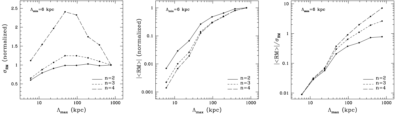
Fig. 3. Normalized dependence of \sigma_{\text{RM}} (left) and |\langle \text{RM} \rangle| (middle) as a function of \Lambda_{\text{max}} , for the three spectral indexes n = 2, 3 and 4 . The right panel shows the ratio |\langle \text{RM} \rangle|/\sigma_{\text{RM}} as a function of \Lambda_{\text{max}} . The minimum magnetic field scale has been fixed at \Lambda_{\text{min}} = 6 \text{ kpc} while \sigma_{\text{RM}} and |\langle \text{RM} \rangle| values have been sampled in 50 \times 50 \text{ kpc}^2 regions.
