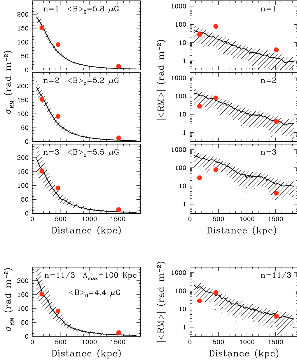
Fig. 8. Best fit of the simulated RM \sigma_{RM} profiles for the cluster A119 (left column panels). The comparison of simulated and observed |<RM>| is shown in right column panels. Solid dots refer to the observed values for the radio galaxies 0053-015, 0053-016 and 3C 29. The best fit to the central magnetic field strength gives \langle B \rangle_0 \approx 5 \mu G . Since the modeled magnetic field strength decreases from the cluster center outward ( \mu \approx 0.5 ), the mean field strength within a spherical volume with radius r = 3 r_c is \langle B \rangle \approx 1.5 \mu G . We find that the spectral index n = 2 gives the best description of the data if the magnetic field power spectrum ranges from a minimum scale of 6 kpc up to a maximum scale of 768 kpc. The fit corresponding to the models with n \leq 1 and n \geq 2 are definitely poorer since the |<RM>|/\sigma_{RM} ratios they predict are too low and too high, respectively. The Kolmogorov spectral index ( n = 11/3 ) gives a reasonable fit to the data only if the maximum scale of the magnetic field fluctuations is about 100 kpc (bottom panels).
