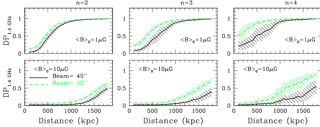
Fig. 5. Simulated 1.4 GHz beam-depolarization as a function of the distance from the cluster center in the case of a varying magnetic field ( \mu = 0.3 ) with a central strength of \langle B \rangle_0 = 1 (top panels) and 10 \mu\text{G} (bottom panels). The simulated cluster is placed at a distance of about 300 Mpc ( z = 0.05 ). Solid and dashed lines refer to a beam size of 45'' and 15'' , respectively. At the distance of the cluster these beam widths correspond to projected linear sizes of about 60 and 20 kpc.
