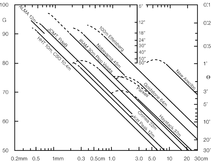
Fig. 7.8 The gain G in dB (left axis) of some high-precision filled aperture radio telescopes is plotted against wavelength \lambda . The Full Width to Half Power, \theta is plotted on the right axis. The ALMA 12 m antennas will have the same properties as the APEX antenna. The curve for these antennas extends to 0.3 mm, and to longer wavelengths, where it joins the curve for the Kitt Peak 12 m antenna which has a lower surface accuracy. The 15 m diameter JCMT (James Clerk Maxwell Telescope) on Mauna Kea and PdeB (IRAM Plateau de Bure interferometer) antennas are also shown. Smaller but highly accurate antennas are a part of the SOFIA and Herschel observatories
