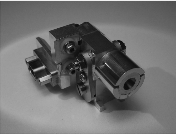
Fig. 5.12 [An ALMA Band 9 SIS mixer] A photo of the feed horn on the right, and the SIS mixer holder on the left. This was built at the Space Research Organization of the Netherlands (SRON). This receiver covers the frequency range 610–720 GHz. This is a tunerless double sideband mixer. This is typical for the sub-mm SIS mixers used in the ALMA instrument
