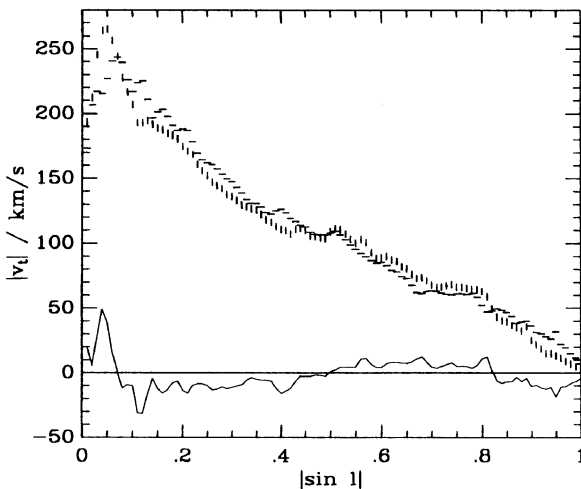
Fig. 13.5 Terminal velocity as function of |\sin l| . “-” for 1st galactic quadrant 0^\circ < l < 90^\circ ; “—” for 4th galactic quadrant 270^\circ < l < 360^\circ , the continuous line shows the difference of the two
