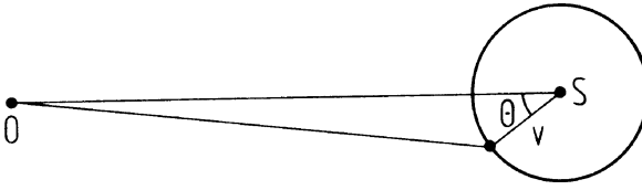
Fig. 11.14 A sketch to illustrate the geometry of light propagation in an expanding source
